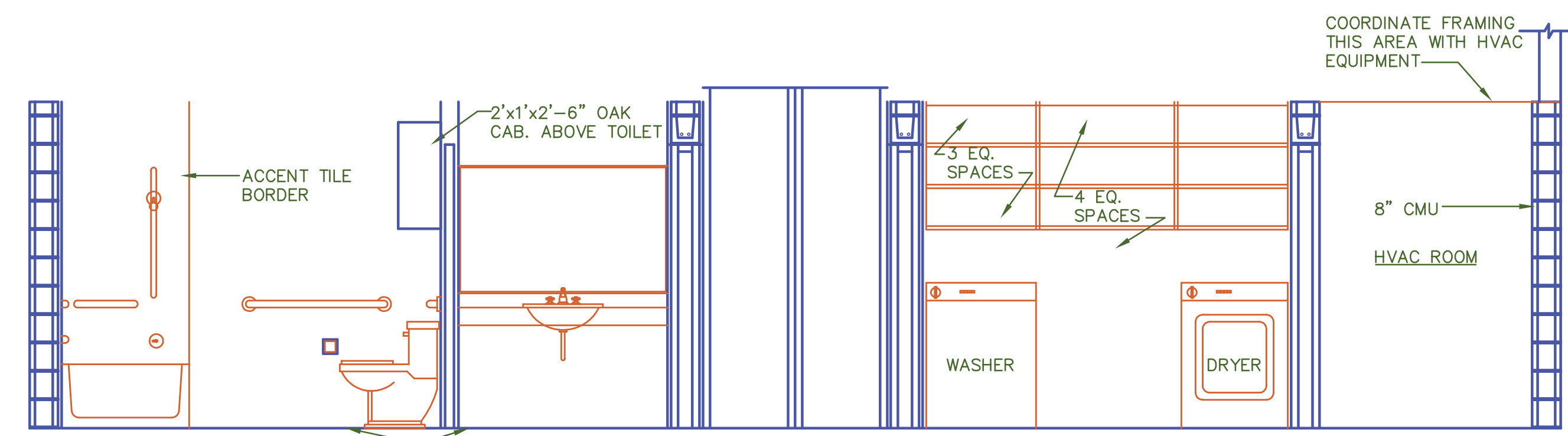
3 HANDICAP RESTROOM AND LAUNDRY ELEVATIONS SCALE: 3/8"=1'-0"
